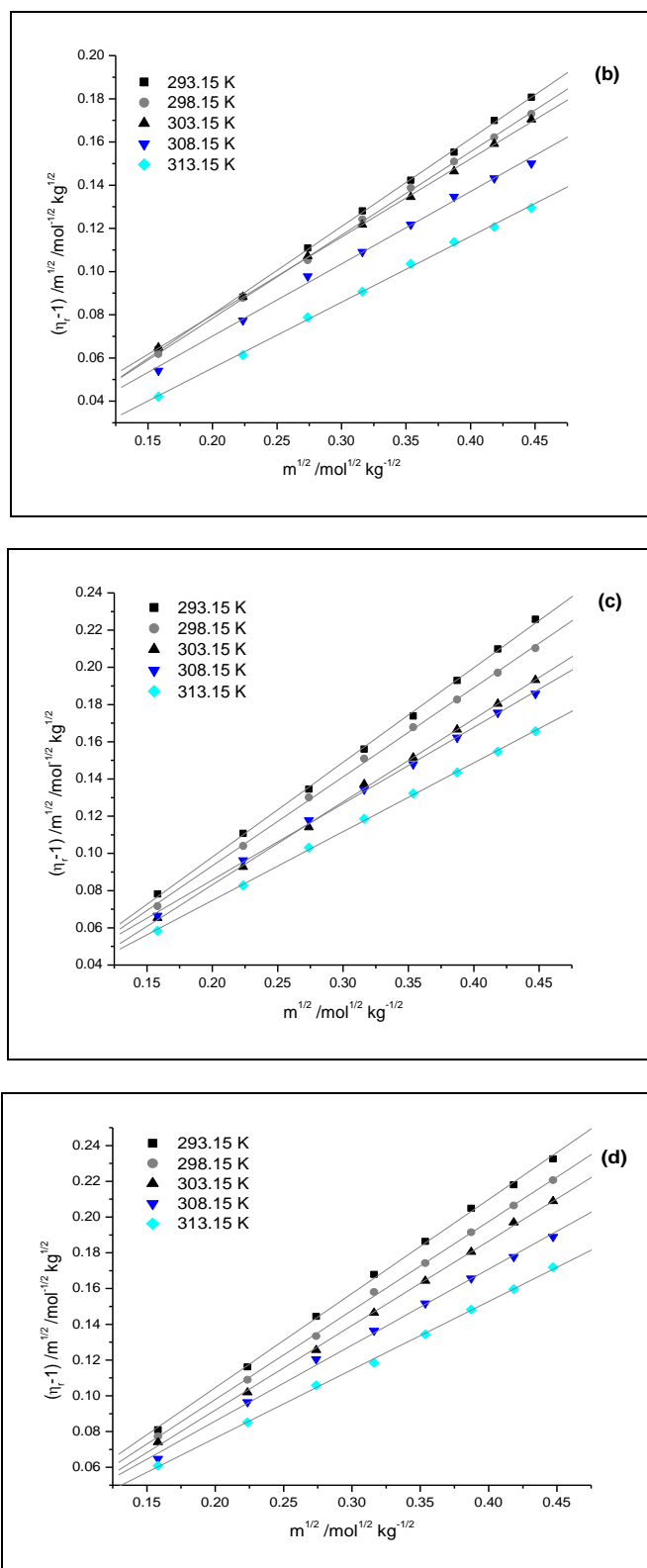
Fig. 2. Variation of reduced viscosity \{(\eta_r - 1)/m^{1/2}\} with molality ( m^{1/2} ) of L-valine in (a) water, (b) 0.1 \text{ mol dm}^{-3} glucose, (c) 0.1 \text{ mol dm}^{-3} sucrose, (d) 0.1 \text{ mol dm}^{-3} lactose, at different temperatures.
