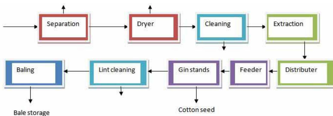
Figure 4-1 Cotton Ginning Process
