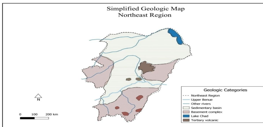
Figure 2: Simplified Geologic Map of the North-East Region
