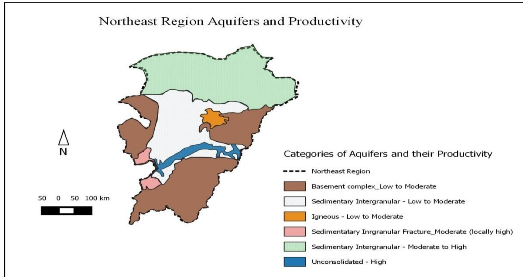
Figure 3: Simplified aquifers distribution of North-East region
