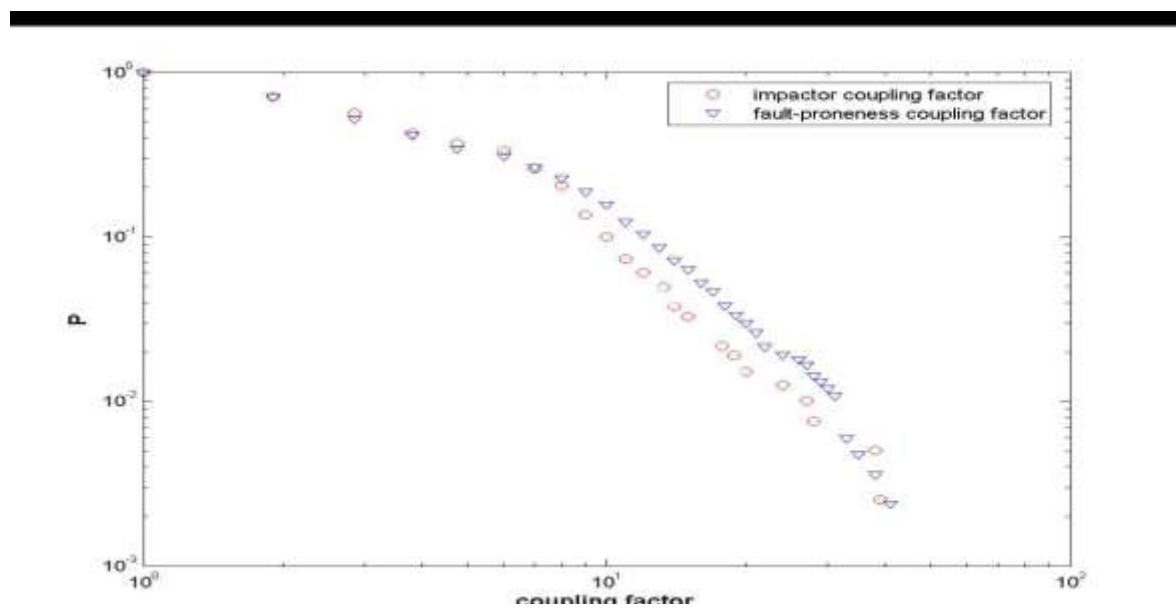
Fig. 5: Log-log plot of the cumulative distribution of reciprocal of impact coupling factor and fault-proneness coupling factor of JEdit in its dynamic coupling network [19]
