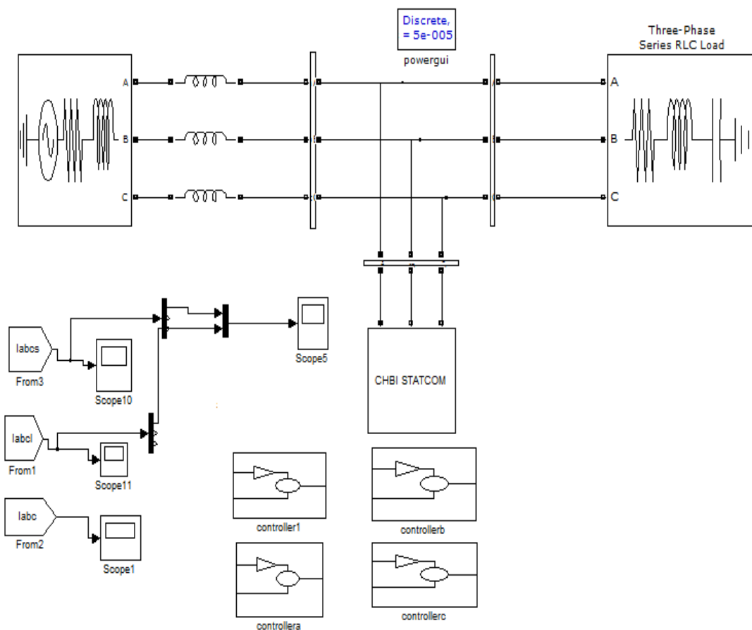
Figure 5 Proposed Model of Multilevel Inverter Based STATCOM
