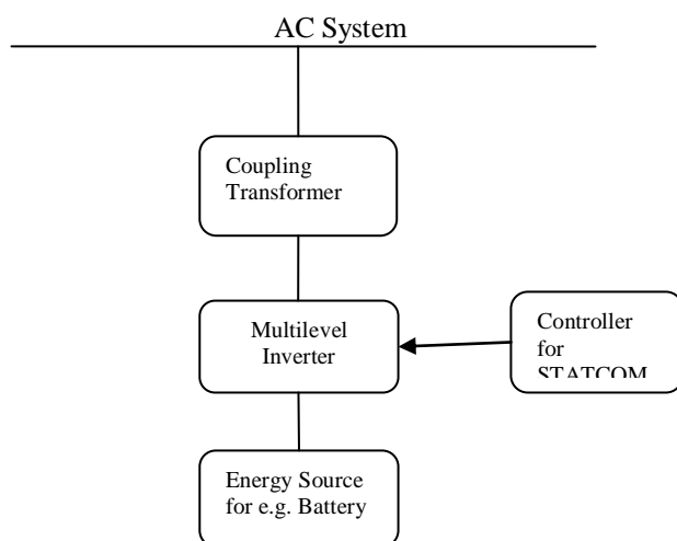
Figure 2 Multilevel Inverter Based STATCOM
