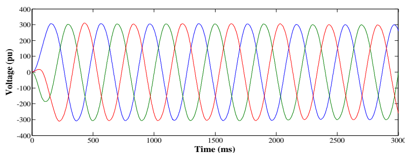
(a) Obtained Voltage in 7 Level CHB STATCOM System
