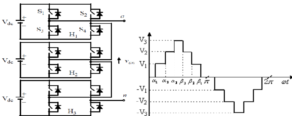
Figure 3 Seven Level CHB Inverter per phase and corresponding output waveform
